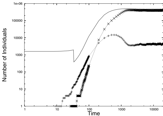
Fig. 1. Time evolution of N_0 (line, original species), N_1 (+, mixed genomes) and N_2 ( \times , new species), for one diploid sexual population simulated on a L \times L square lattice with L = 800 and N_0 = 1600 individuals.
